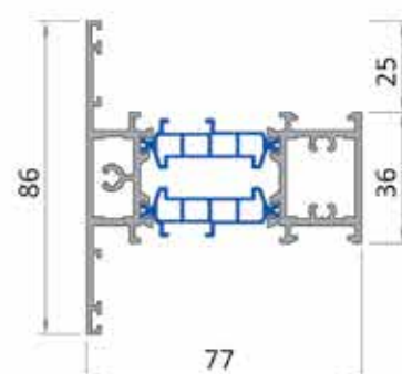
Mullion profile RP 85.33 1990 g/m
