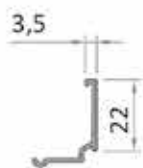
Glazing bead RP 40.03 165 g/m
