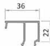
Glazing bead RP 85.36 380 g/m
