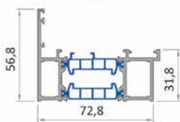
Frame profile RP 85.01 1700 g/m
