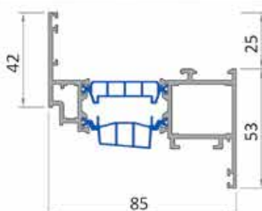
Sash profile RP 85.21 1800 g/m
