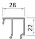
Glazing bead RP 85.28 345 g/m
