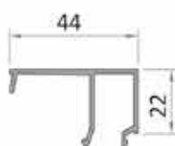
Glazing bead RP 85.44 420 g/m
