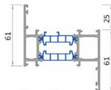
Frame profile RP 85.05 1830 g/m
