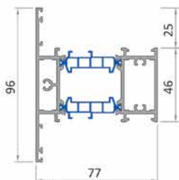
Mullion profile RP 85.37 2190 g/m
