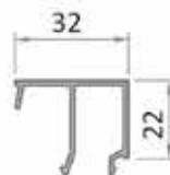
Glazing bead RP 85.32 360 g/m
