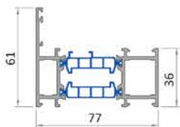
Frame profile RP 85.01 1700 g/m
