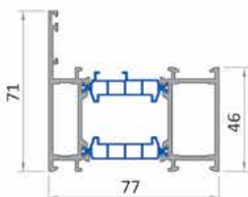
Frame profile RP 85.02 1890 g/m
