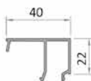
Glazing bead RP 85.40 400 g/m
