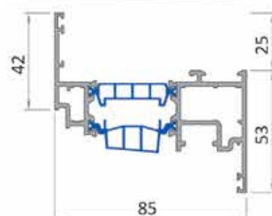
Sash profile RP 85.22 1830 g/m
