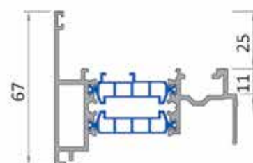
Mullion profile RP 85.33 1990 g/m
